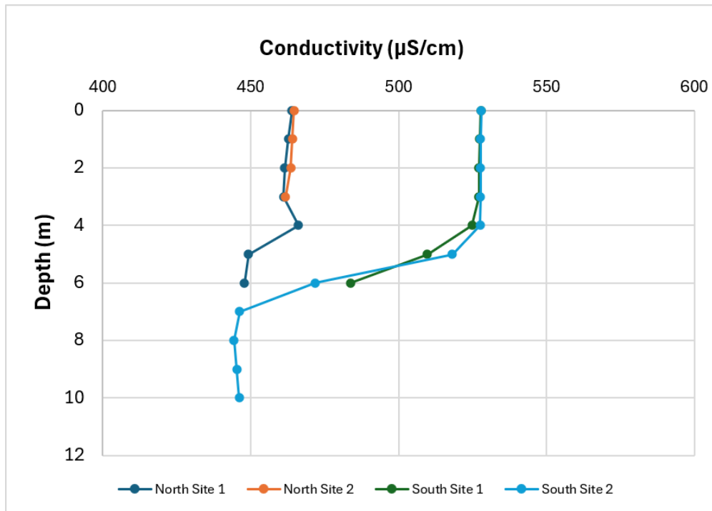
Figure 4. Graph of conductivity measurements (reported in \mu\text{S}/\text{cm} ) collected with depth on June 16, 2026
