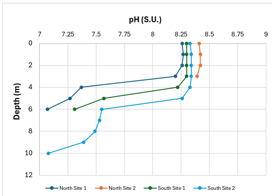
Figure 1. Graph of pH measurements (reported in standard units) collected with depth on June 16, 2026
